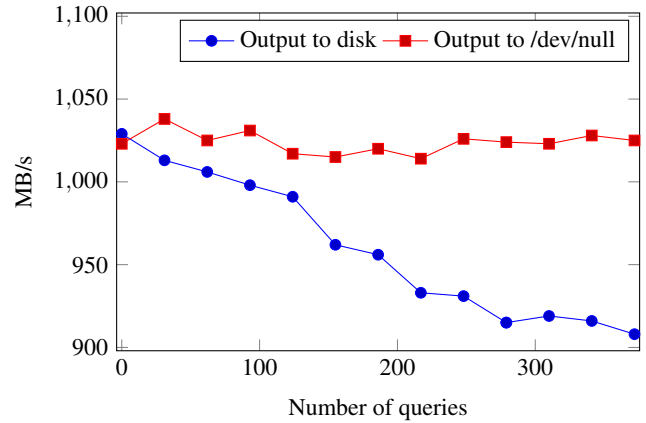
Figure 6. Decrease in read throughput as queries are added, comparing writing the output to disk and writing to /dev/null .
